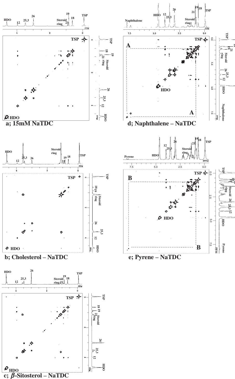
Fig. 4. Contour plots of the saturated solubilizes of NaTDC solutions (15 mM) from the ROESY measurements. The condition of each solution is as follows. a: pure micellar solution of NaTDC (15 mM); b: saturated cholesterol–NaTDC; c: saturated \beta -sitosterol–NaTDC; d: saturated naphthalene–NaTDC; and e: saturated pyrene–NaTDC. The concentrations of the solubilizes correspond with those shown in Fig. 2. A and B in Figs. 4d and 4e indicate cross-peaks between naphthalene and the 19-methyl group and pyrene and the 19-methyl group, respectively.
